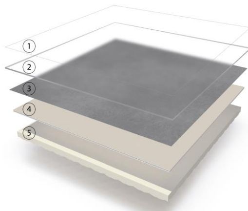
Figure 1: Typical construction
