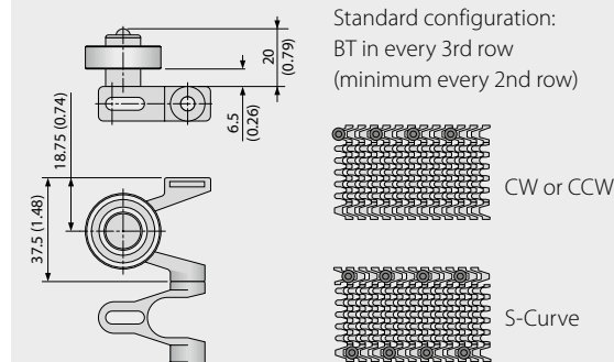
Variant specific dimensions [mm (in)]
