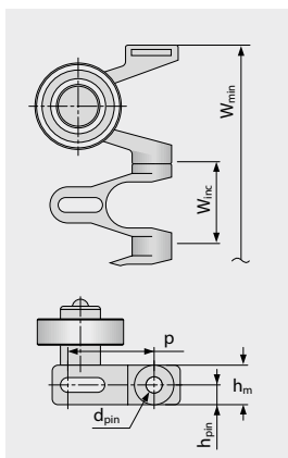
Variant specific dimensions [mm (in)]
