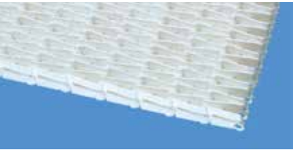
S2 | 57% open | Raised Rib
