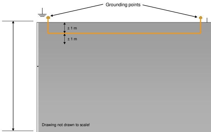
Picture 2 – Copper strip layout for rooms > 50 \text{ m}^2 , alternative A
