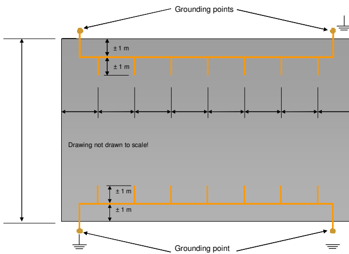
Picture 3 – Copper strip layout for rooms > 50 \text{ m}^2 , alternative B
