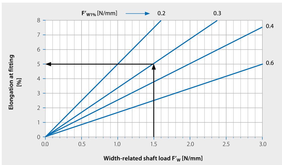
Diagram 1: Identifying the minimum shaft load
