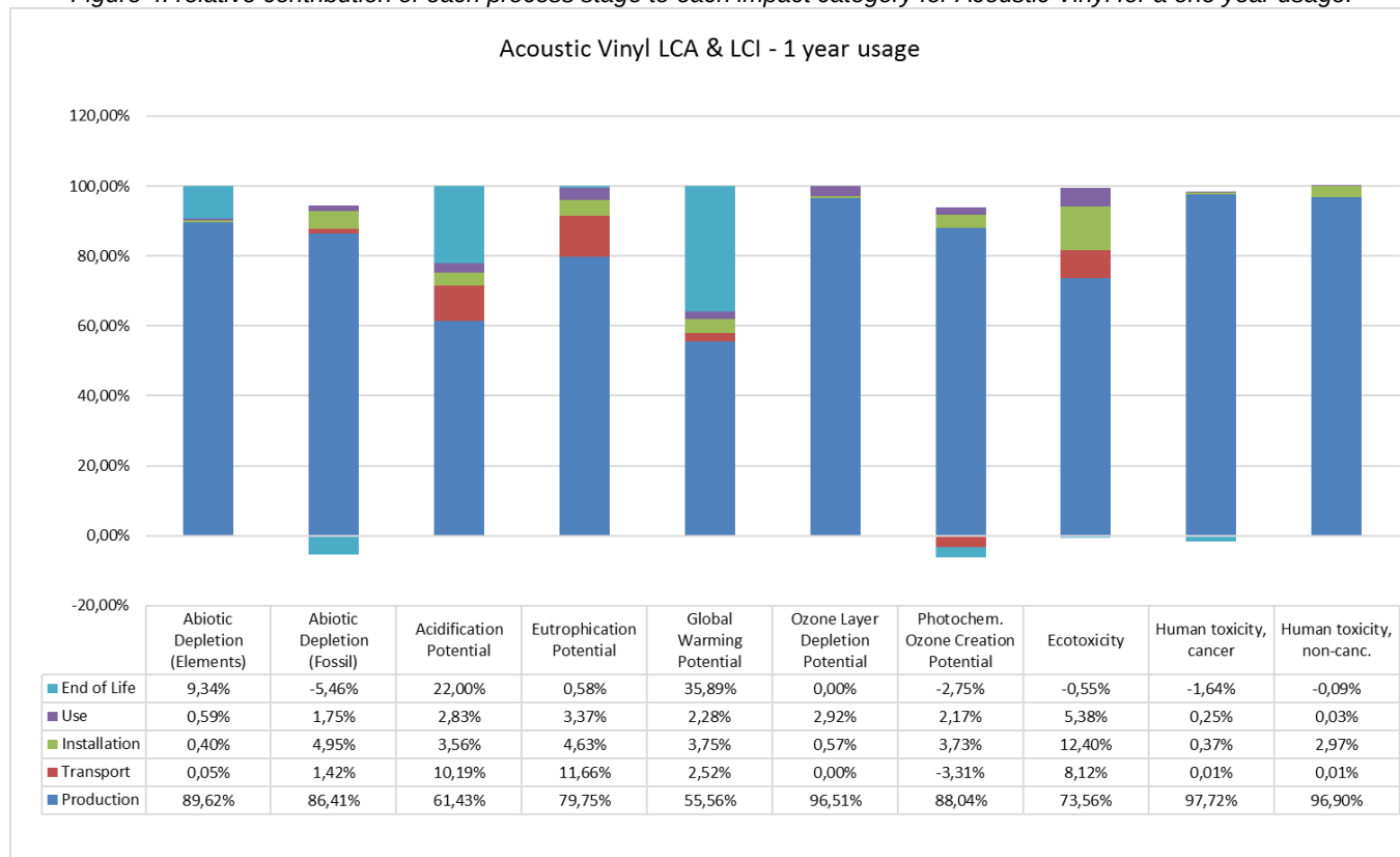
Figure 4: relative contribution of each process stage to each impact category for Acoustic Vinyl for a one year usage.
