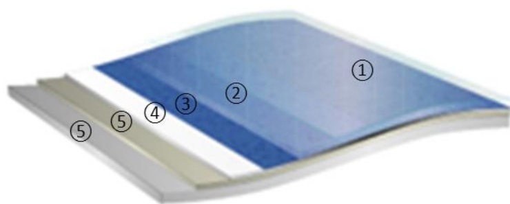
Figure 1 : Schematic build-up of Acoustic Vinyl
