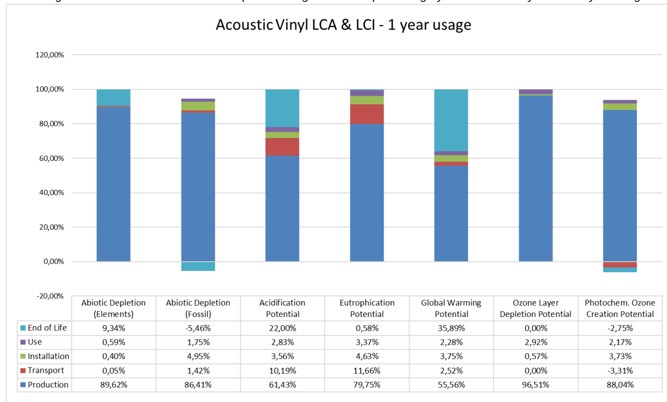
Figure 3: relative contribution of each process stage to each impact category for Acoustic Vinyl for a one year usage.
