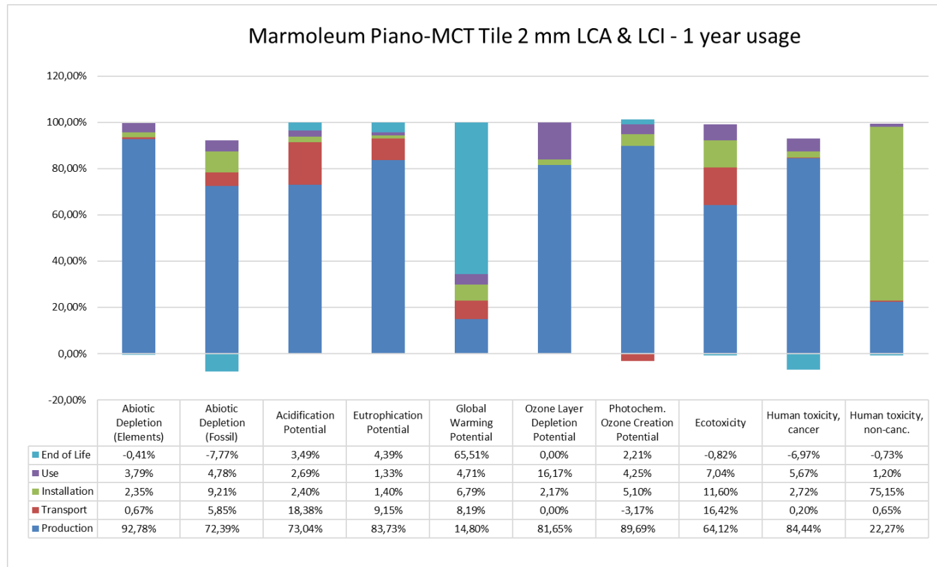
Figure 5: relative contribution of each process stage to each impact category for Marmoleum Modular Piano – MCT for a one year usage.
