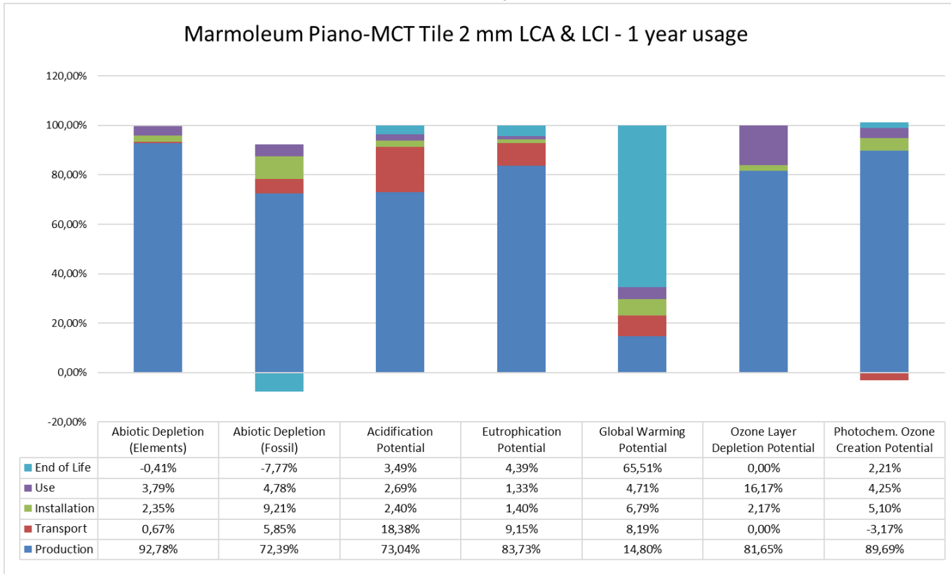
Figure 4: relative contribution of each process stage to each impact category for Marmoleum Modular Piano – MCT for a one-year usage.
