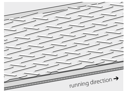
Staggered stud (VN) peeled off at belt edges (scale 1:5)
