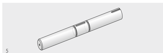
Fixation of the sprocket with retainer rings in accordance with DIN 471 (Seeger circlip ring).
