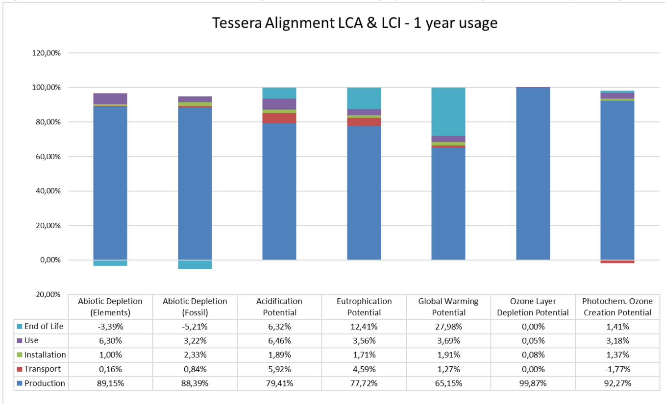
Figure 4: relative contribution of each process stage to each impact category for Tessera Alignment for a one year usage.
