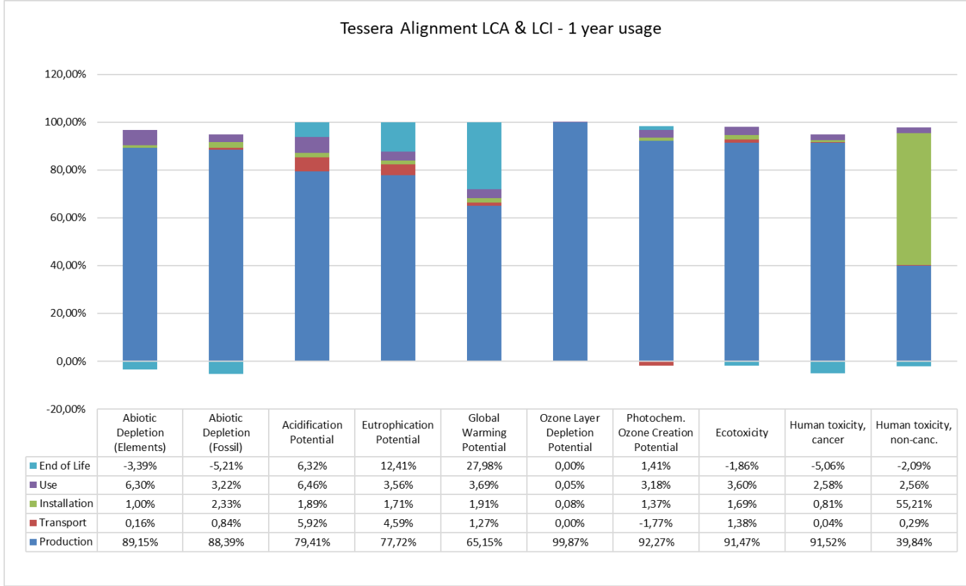
Figure 5: relative contribution of each process stage to each impact category for Tessera Alignment for a one year usage.
