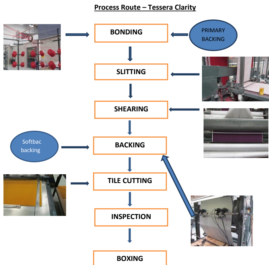
Figure 2: Production process of Tessera Clarity
