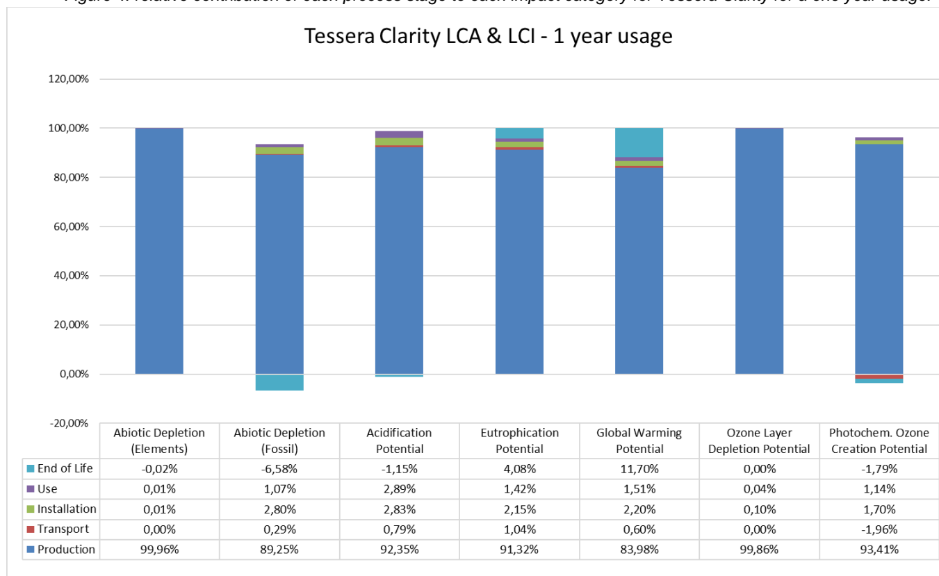
Figure 4: relative contribution of each process stage to each impact category for Tessera Clarity for a one year usage.
