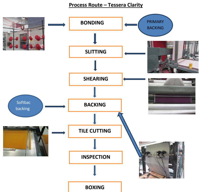
Figure 2: Production process of Tessera Clarity
