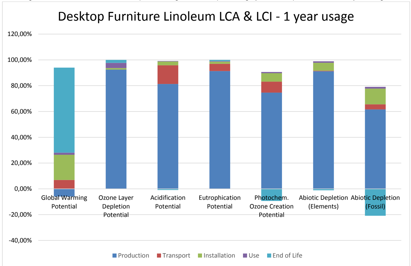
Figure 4: relative contribution of each process stage to each impact category for Desktop 2.0 mm for a one year usage.
