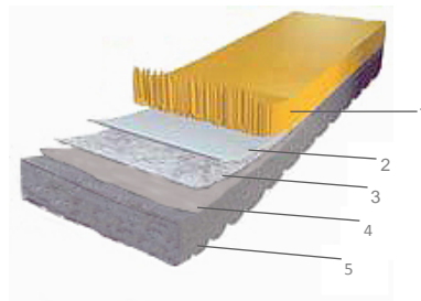
Figure 1: Illustration of Flotex Tile
