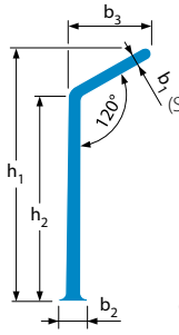
SF-SB (Short bent (curvado corto))
