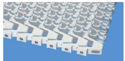
S5 | 45 % open | Nub Top
