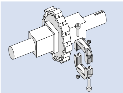
Siegling Prolink Retainer Rings provides a quick, easy and reliable solution for fixing the sprocket (see page I-206 for details).
