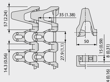
Variant specific dimensions [mm (in)]
