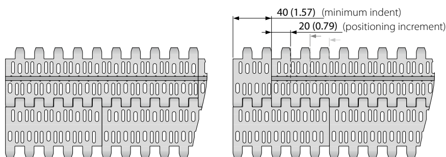
Standard configuration S6.1-23 NCL PMU
