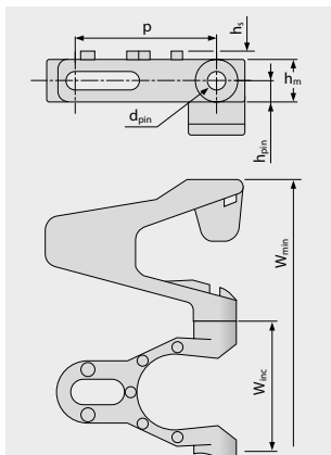
Variant specific dimensions [mm (in)]
