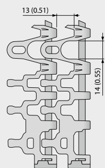
Variant specific dimensions [mm (in)]
