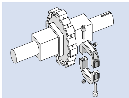
Siegling Prolink Retainer Rings provides a quick, easy and reliable solution for fixing the sprocket (see page I-216 for details).
