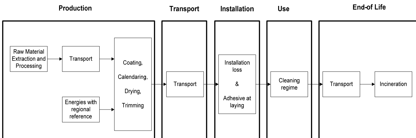
Figure 3: Flow chart of the Life Cycle Assessment
