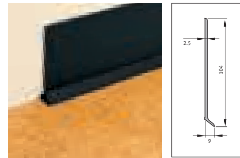
Article reference : PX A 104 mm high flexible sit-on cove skirting.
