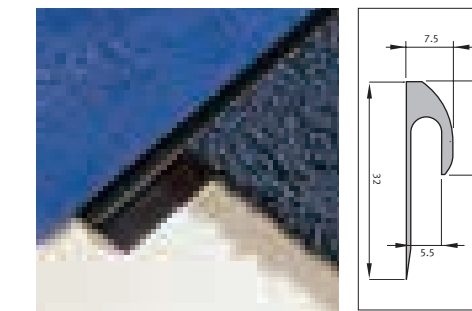
Article reference : WX Covering transition strip for use with carpet, carpet tile or entrance mats to resilient flooring.
