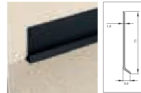
Article reference : PY A 75 mm high flexible sit-on PVC cove skirting.
