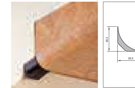
Article reference : PS An extruded cove former with a 30 mm internal radius for use with linoleum floor finishes.
