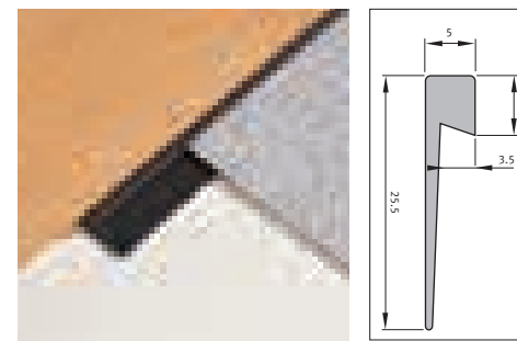
Article reference : WA Edging strip for transition between resilient flooring and carpet. May also be used as a decorative and hygienic capping strip for coved or Marmoform S skirting.
