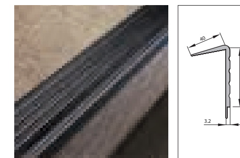
Article reference : TJ Heavy-duty stairnosings for situations where intensive traffic is expected.
