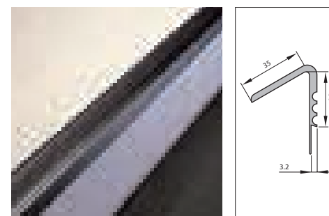
Article reference : TA Standard size general-purpose stairnosings; top surface is ribbed for improved slip-resistance and safety.
