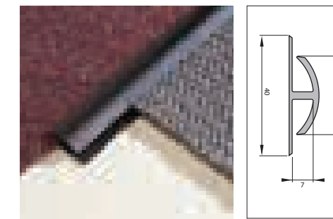
Article reference : WO Junction strip for use between different carpet finishes or between carpets and entrance mats.
