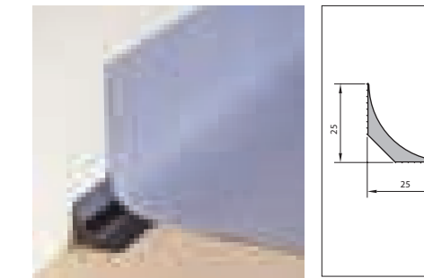
Article reference : PR An extruded cove former with a 25 mm internal radius for use with vinyl floor finishes.
