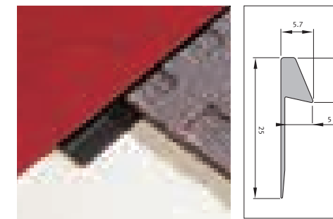
Article reference : WB Transition strip for use with carpet, carpet tile or resilient flooring. May also be used for forming curved transitions, due to its horizontal flexibility.
