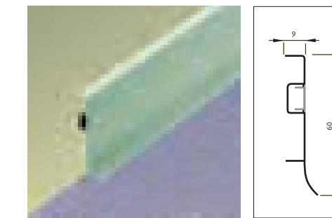
Article reference : PV Ventilated skirtings allow good ventilation of the substrate, especially when an impervious floor is installed (e.g. vinyl flooring, or foil or foam under floorings). After the floor is installed, the profile can be mounted on the wall using screws. A decorative strip covers the screw fixings. Length : 3 m Number per carton box : 20 Colours : 17 or 20 (white)
