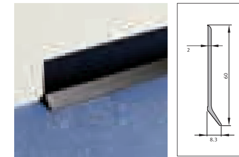
Article reference : PZ A 60 mm high flexible sit-on PVC cove skirting.
